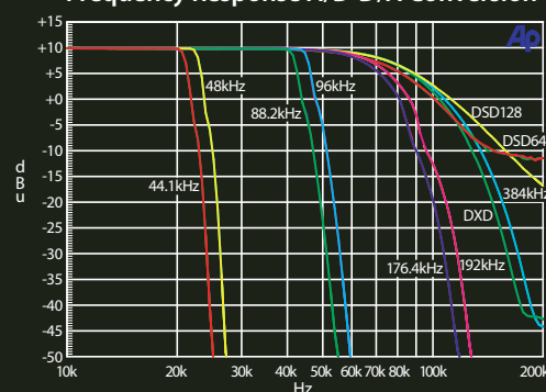
Frequency Response A/D-D/A Conversion
