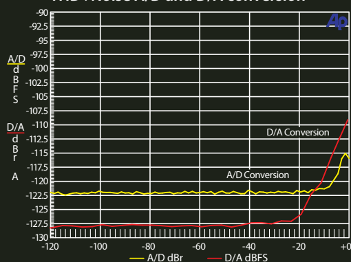
THD+Noise A/D and D/A conversion
